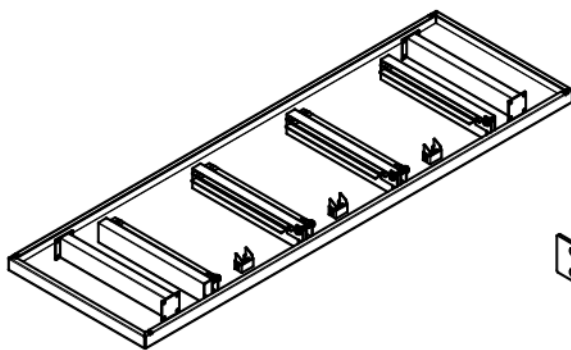
A) WORK BENCH TOP (1PC)
