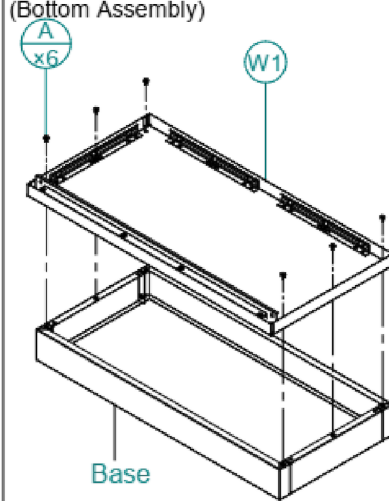
Step 2 (Bottom Assembly)
